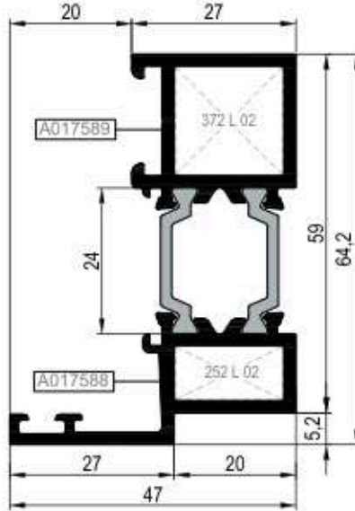
RWT64 SİSTEM ADAPTÖRÜ ADAPTER FOR RWT64 SYSTEM
