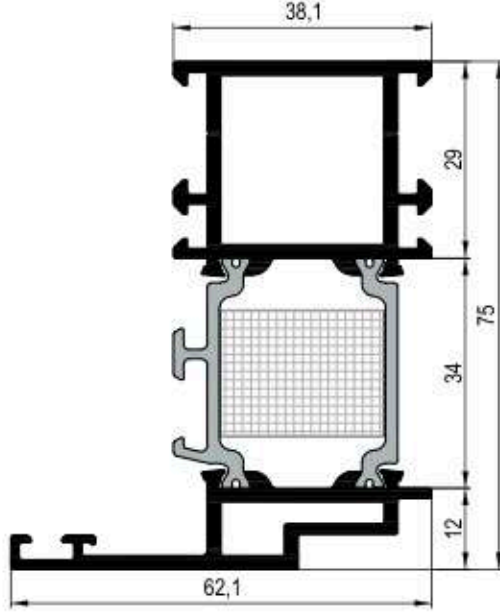
RWT75 SİSTEM ADAPTÖRÜ ADAPTER FOR RWT75 SYSTEM
